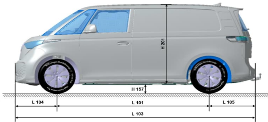
Fig. 1. Example vehicle dimensions of ID. Buzz Cargo (acc. to DIN 70200, P1). The dimensions are given in the basic data table below.
