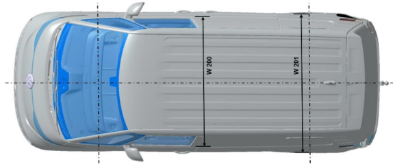
Fig. 1. Example vehicle dimensions of ID. Buzz Cargo (acc. to DIN 70200, P1). The dimensions are given in the basic data table below.
