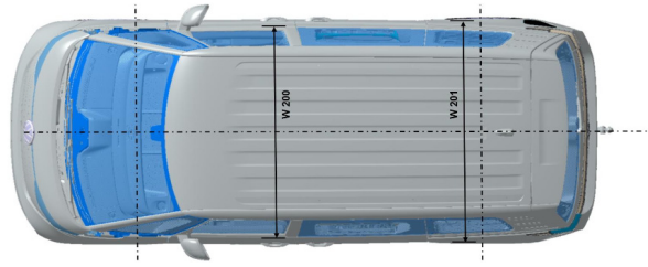
Fig. 1: Example vehicle dimensions of the ID Buzz People (acc. to DIN 70020, P3) The dimensions are given in the basic data table below.
