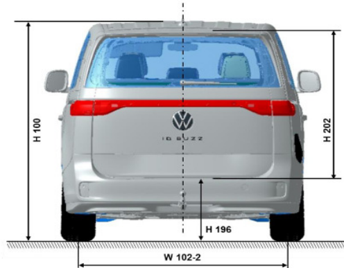
Fig. 2: Example vehicle dimensions of the ID Buzz People (acc. to DIN 70020, T1) The dimensions can be found in the basic data table below.
