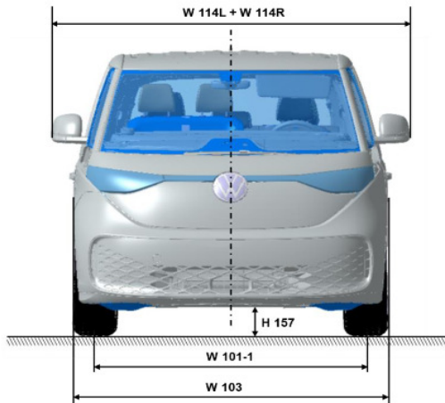
Fig. 2: Example vehicle dimensions of the ID Buzz People (acc. to DIN 70020, T1) The dimensions can be found in the basic data table below.
