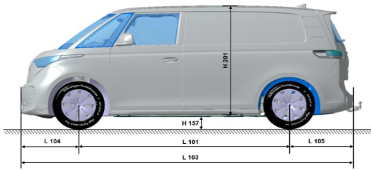
Fig. 1: Example vehicle dimensions of ID Buzz Cargo (acc. to DIN 70020, P1) The dimensions are given in the basic data table below.
