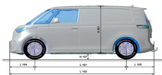
Fig. 1: Example vehicle dimensions of ID Buzz Cargo (acc. to DIN 70020, P2) The dimensions are given in the basic data table below.
