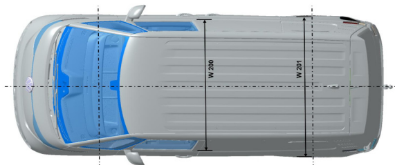
Fig. 1: Example vehicle dimensions of ID Buzz Cargo (acc. to DIN 70020, P2) The dimensions are given in the basic data table below.
