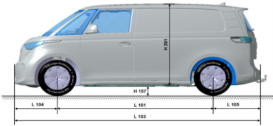
Fig. 1: Example vehicle dimensions of ID Buzz Cargo (acc. to DIN 70020, P1) The dimensions are given in the basic data table below.
