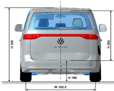
Fig. 2: Example vehicle dimensions of the ID Buzz People (acc. to DIN 70020, T1) The dimensions can be found in the basic data table below.
