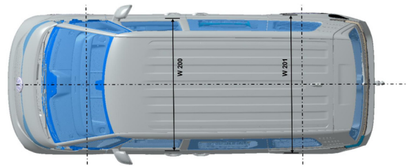
Fig. 1: Example vehicle dimensions of the ID Buzz People (acc. to DIN 70020, P1) The dimensions are given in the basic data table below.
