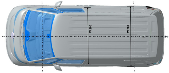
Fig. 1: Example vehicle dimensions of ID. Buzz Cargo (acc. to DIN 70202, P1). The dimensions are given in the basic data table below.
