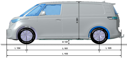
Fig. 1: Example vehicle dimensions of ID. Buzz Cargo (acc. to DIN 70202, P1). The dimensions are given in the basic data table below.
