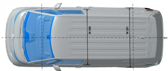
Fig. 1: Example vehicle dimensions of ID Buzz Cargo (acc. to DIN 70020, P1) The dimensions are given in the basic data table below.
