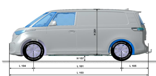
Fig. 1: Example vehicle dimensions of ID Buzz Cargo (acc. to DIN 70020, P1) The dimensions are given in the basic data table below.
